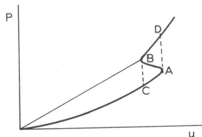
FIG. 21. Hugoniot curve with unstable region 1 < j^2 (dV/dP)_H , between A and B: (a) P - V plane, (b) P - u plane. Point A is relative maximum in E' along H ; B is relative minimum.
